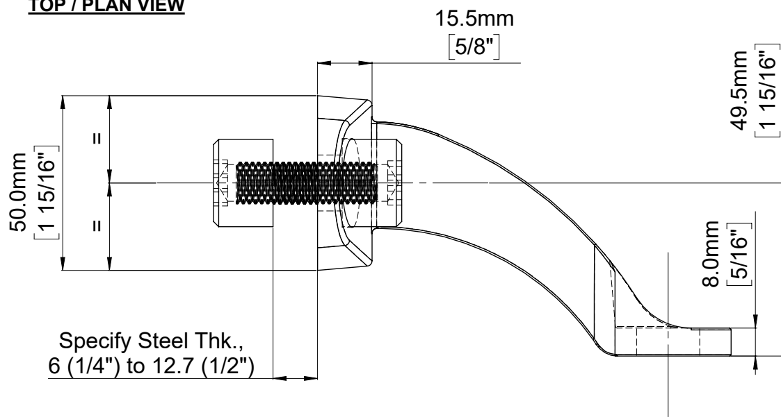
ELEVATION VIEW
