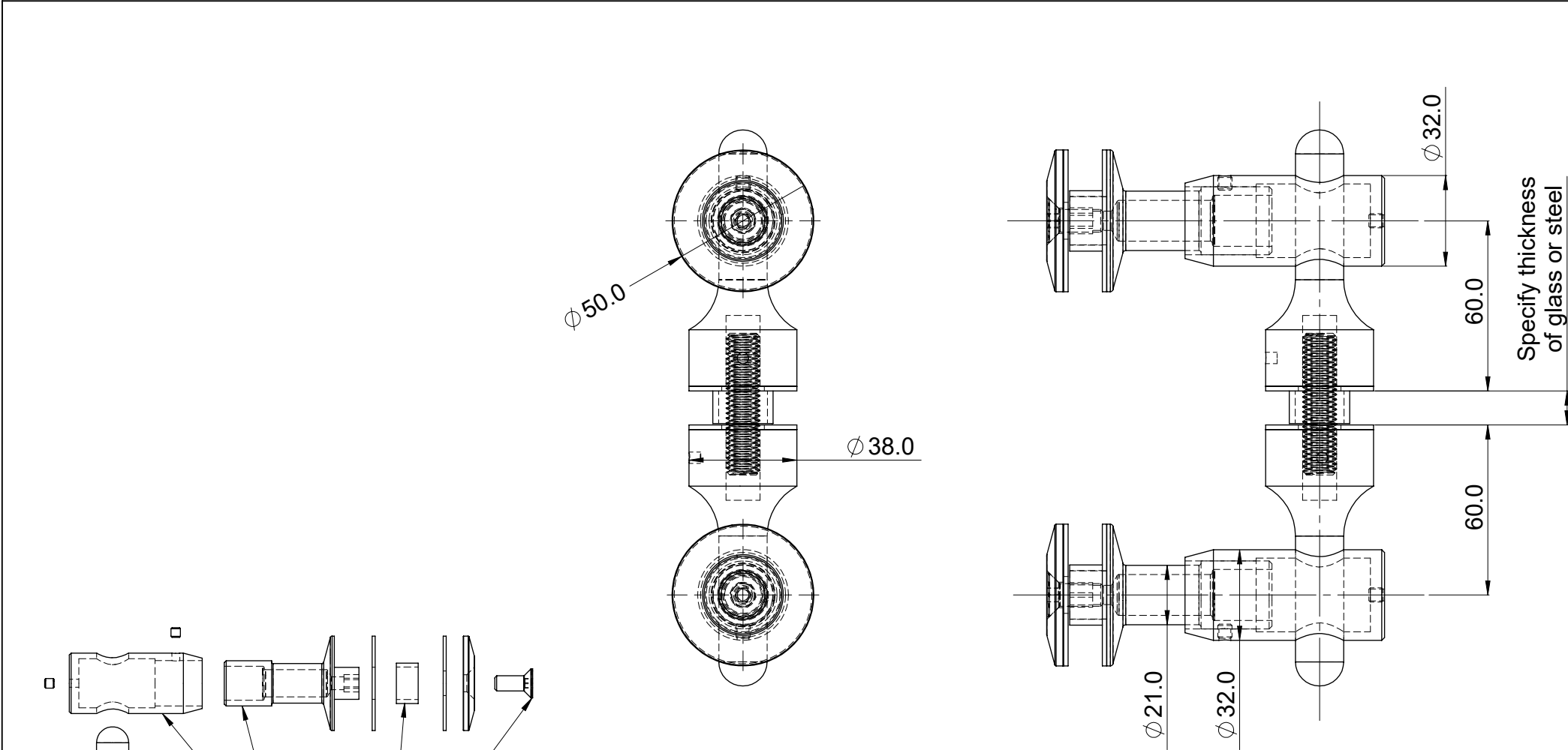
FRONT VIEW
