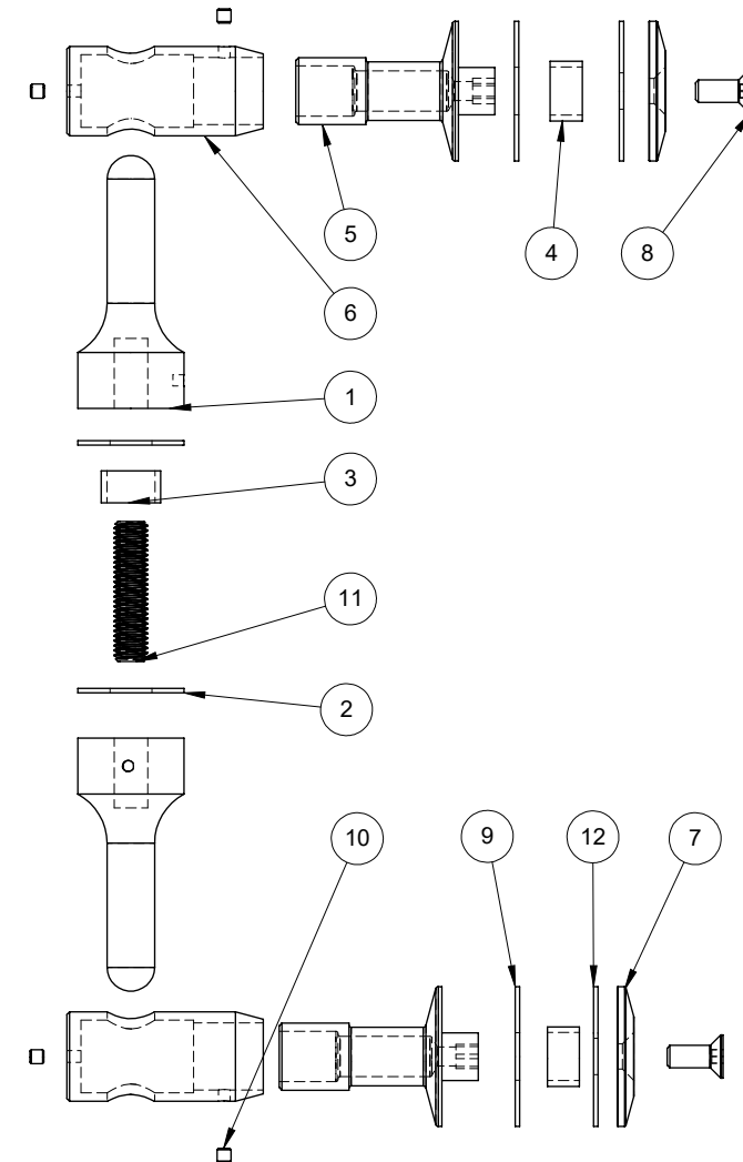
EXPLODED VIEW
