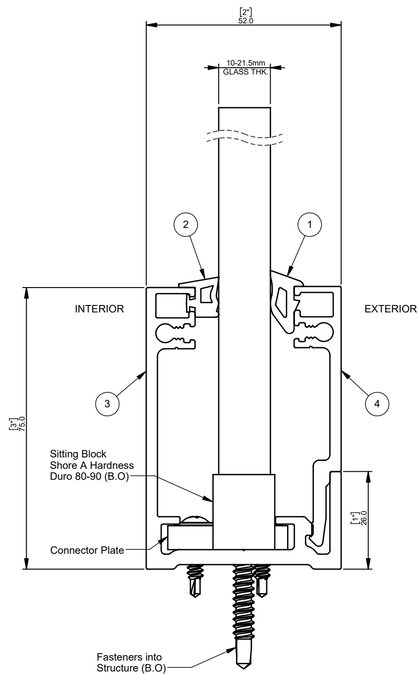
FRONT VIEW
