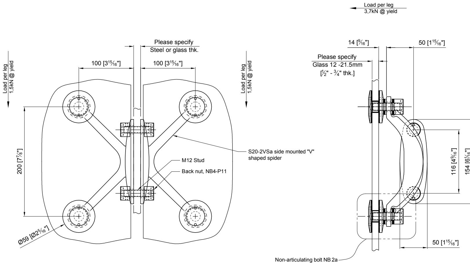
FRONT VIEW
