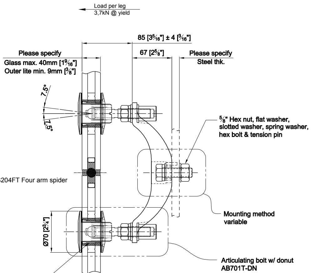
SIDE VIEW
