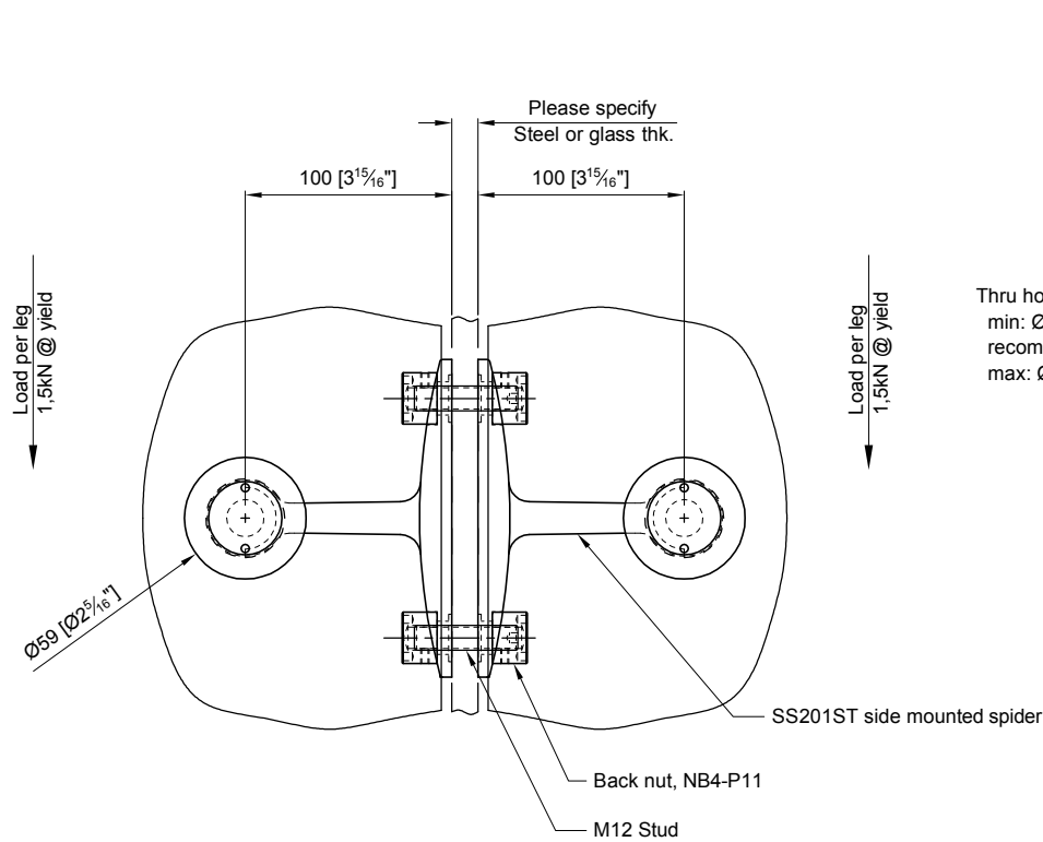
FRONT VIEW
