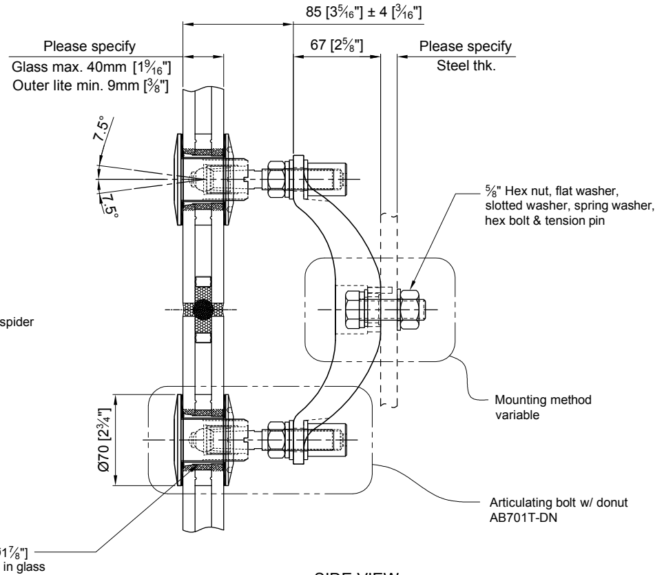
SIDE VIEW
