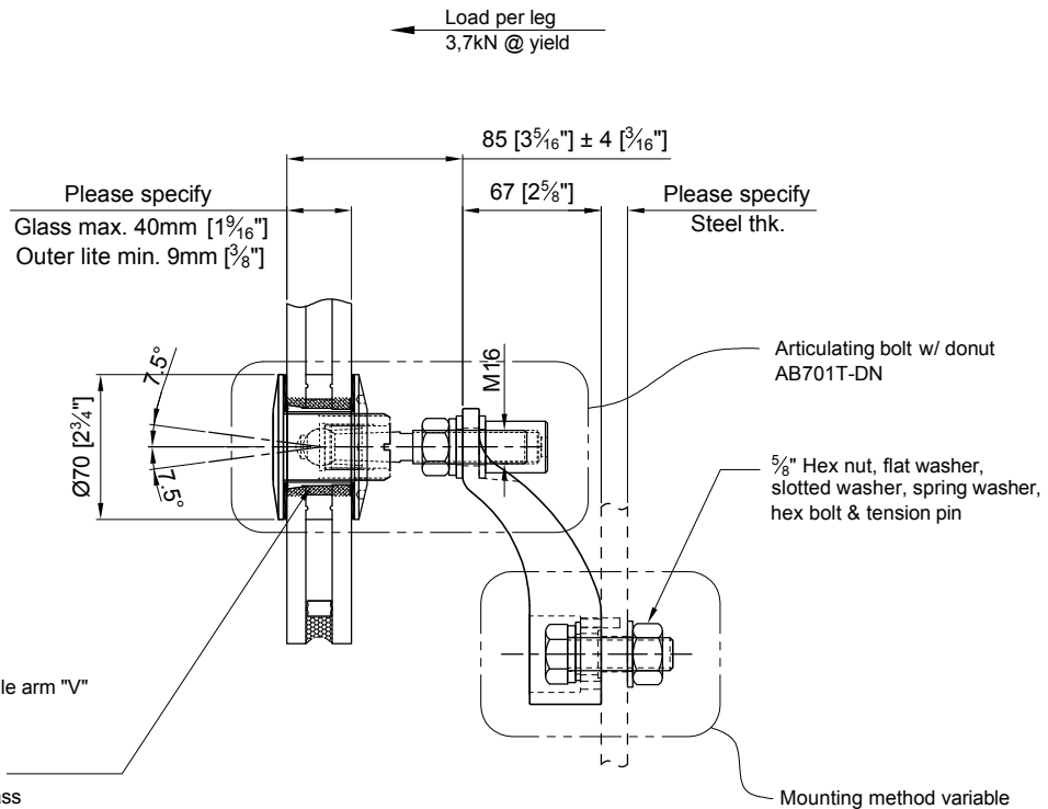
SIDE VIEW
