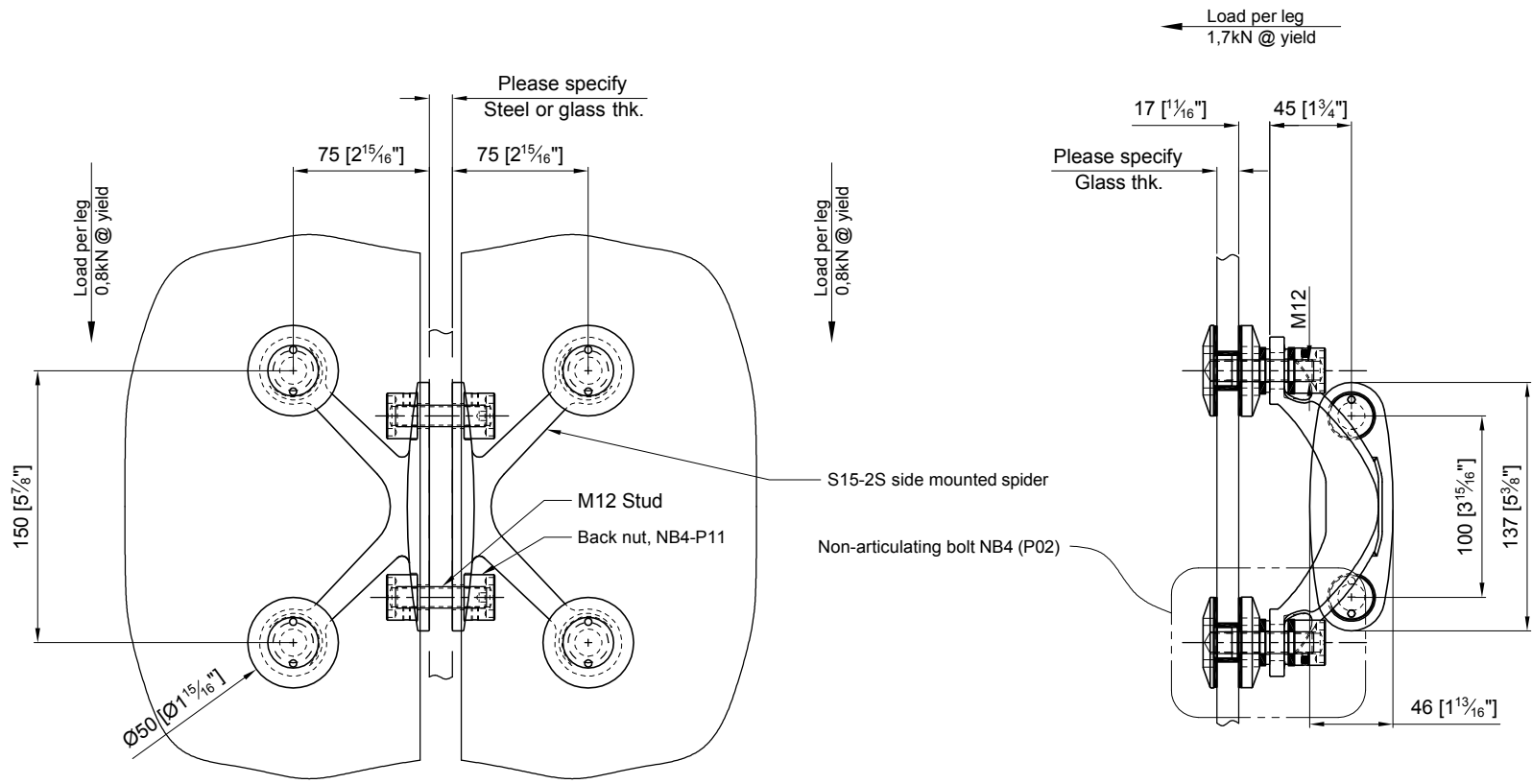
FRONT VIEW
