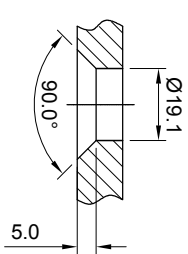
Hole details - monolythic
