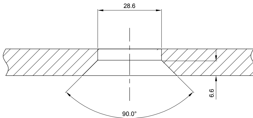
Hole details
