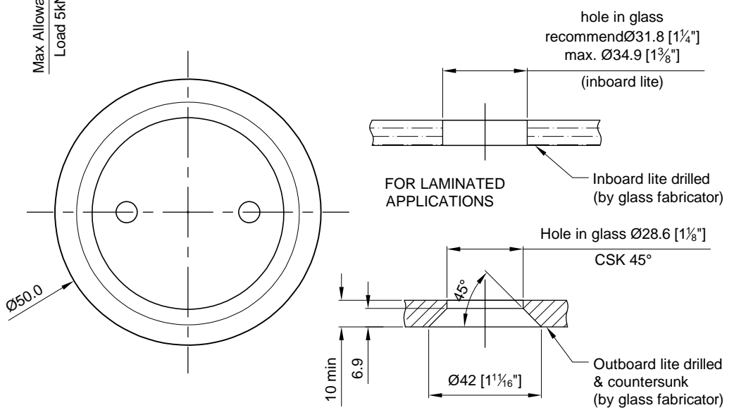
HOLE IN GLASS SCALE: 1:2
